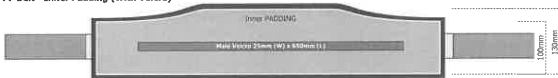
PP Belt - Inner Padding (With Velcro)
