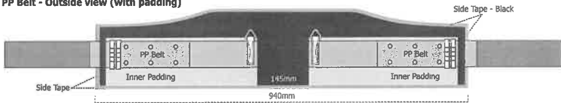
PP Belt - Outside view (with padding)
